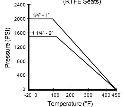
103 Pressure / Temperature Chart (RTFE Seats)
